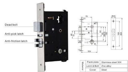
Mortise ANSI-S(zinc alloy latches)
