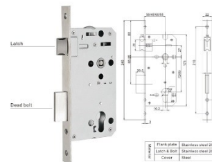
Mortise European(3072/85,4072/85, 4572/85,5072/85,5572/85,6072/85)
